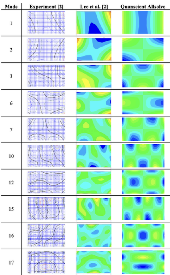
Fig. 4: Comparison of selected modes with experimental modal analysis and finite element analysis from Lee et al. [2]. The deviations in mode shapes are attributed to neglecting accelerometer mass and use of simple gradient-based optimization, leading to a local optimum rather than a global one.
