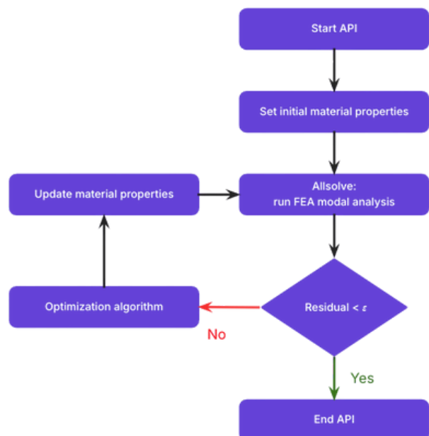
Fig. 2: API optimization workflow.
